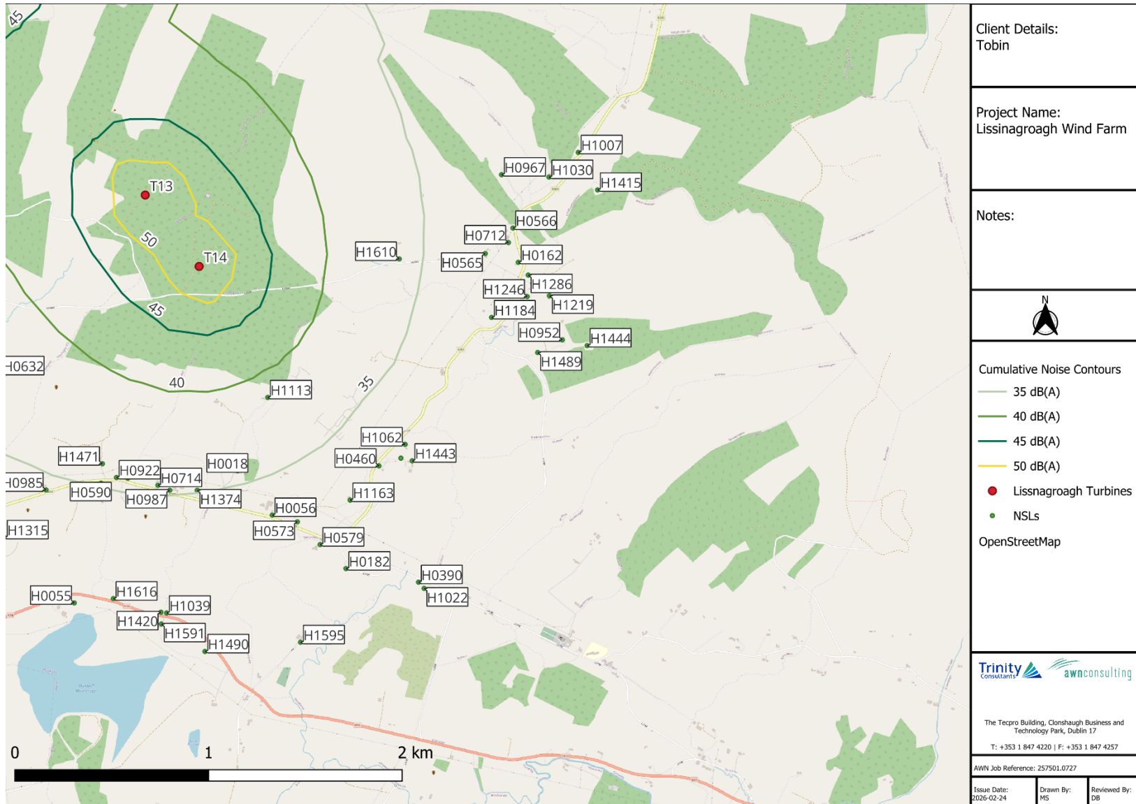
Figure 12-8-5. Predicted Cumulative Noise Contours Detail 5
