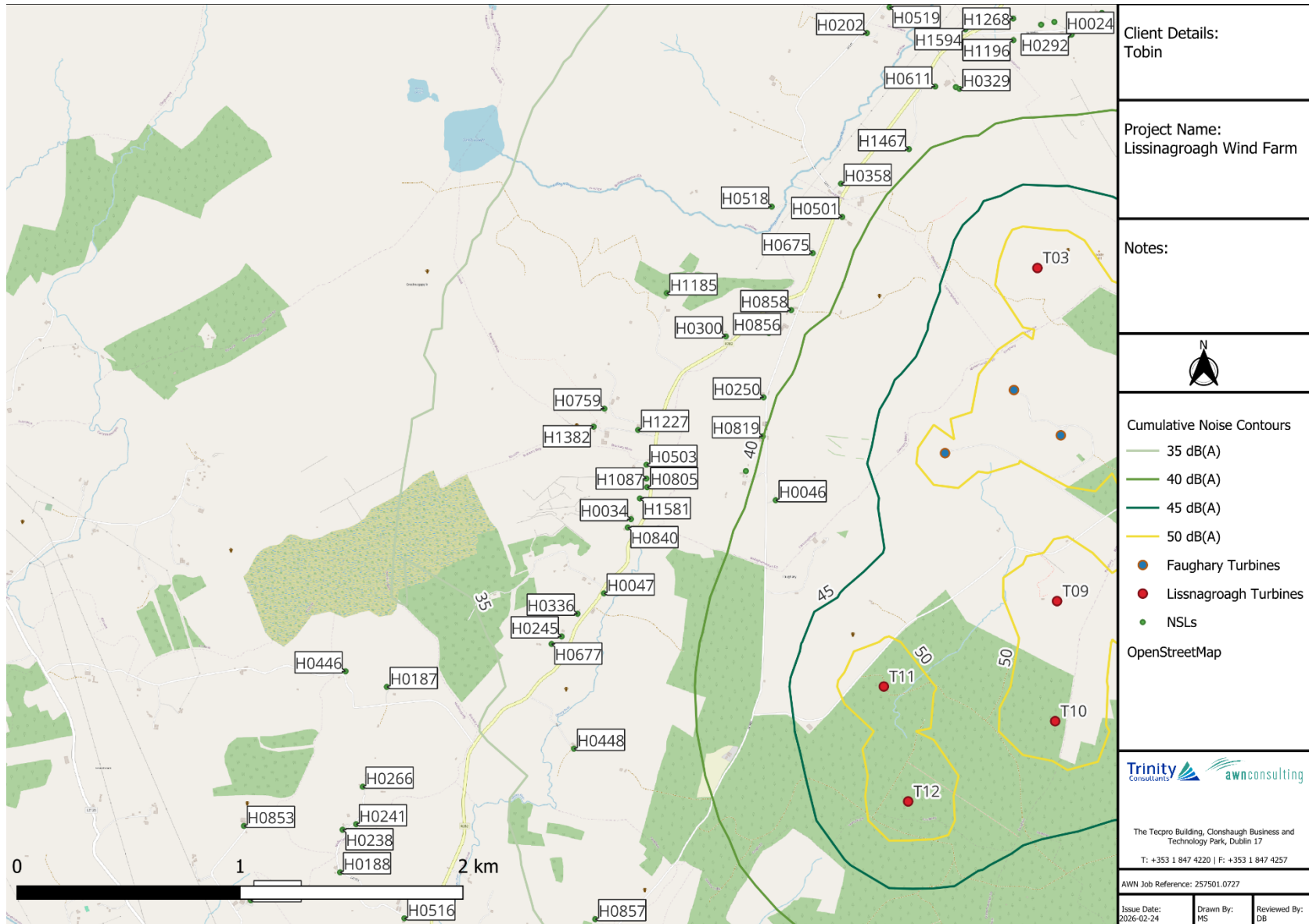
Figure 12-7-3. Predicted Cumulative Noise Contours Detail 2
