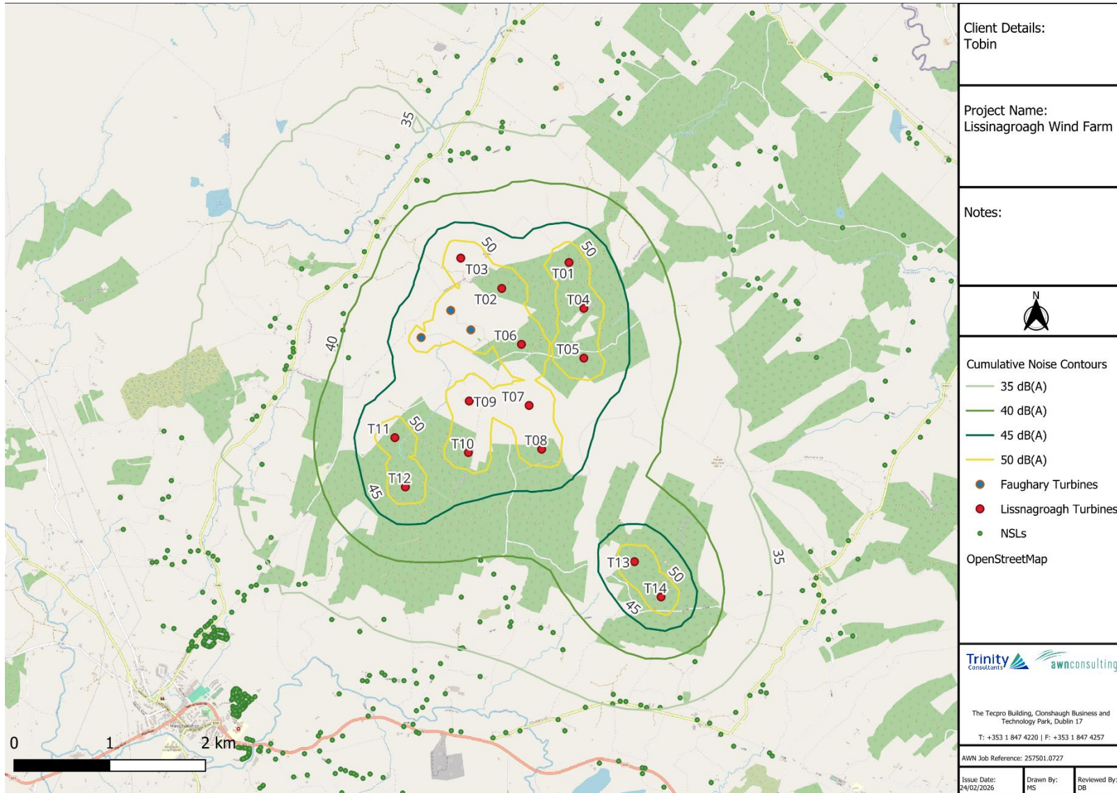
Figure 12-7-1. Predicted Cumulative Noise Contours Overall
