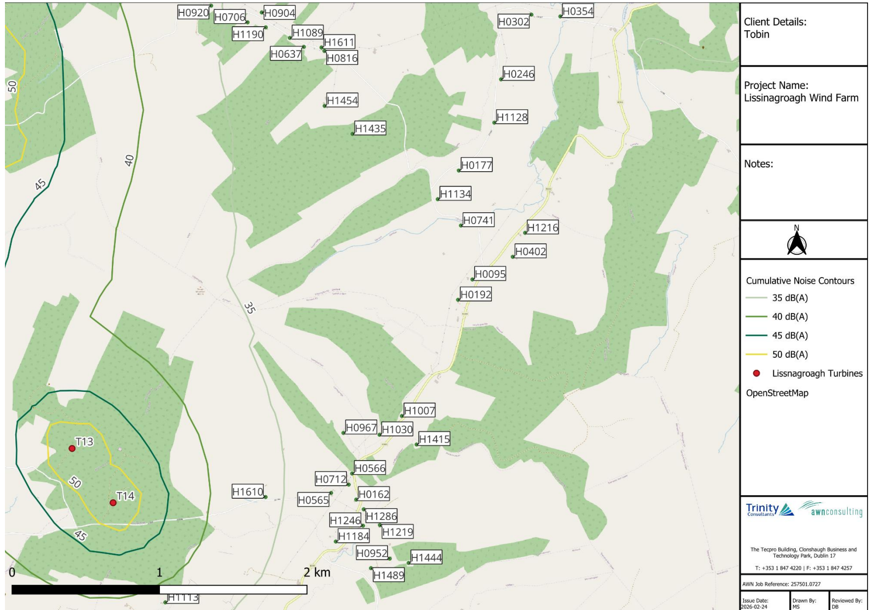
Figure 12-8-5. Predicted Cumulative Noise Contours Detail 6
