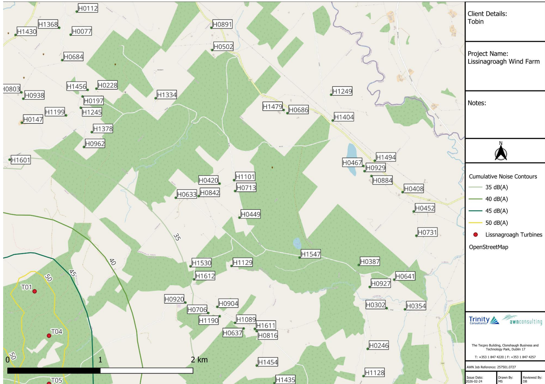
Figure 12-8-5. Predicted Cumulative Noise Contours Detail 7
