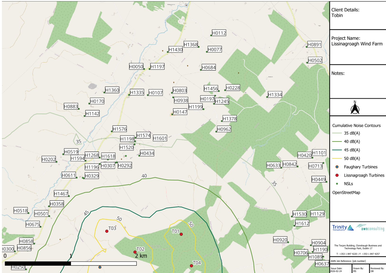
Figure 12-7-2. Predicted Cumulative Noise Contours Detail 1
