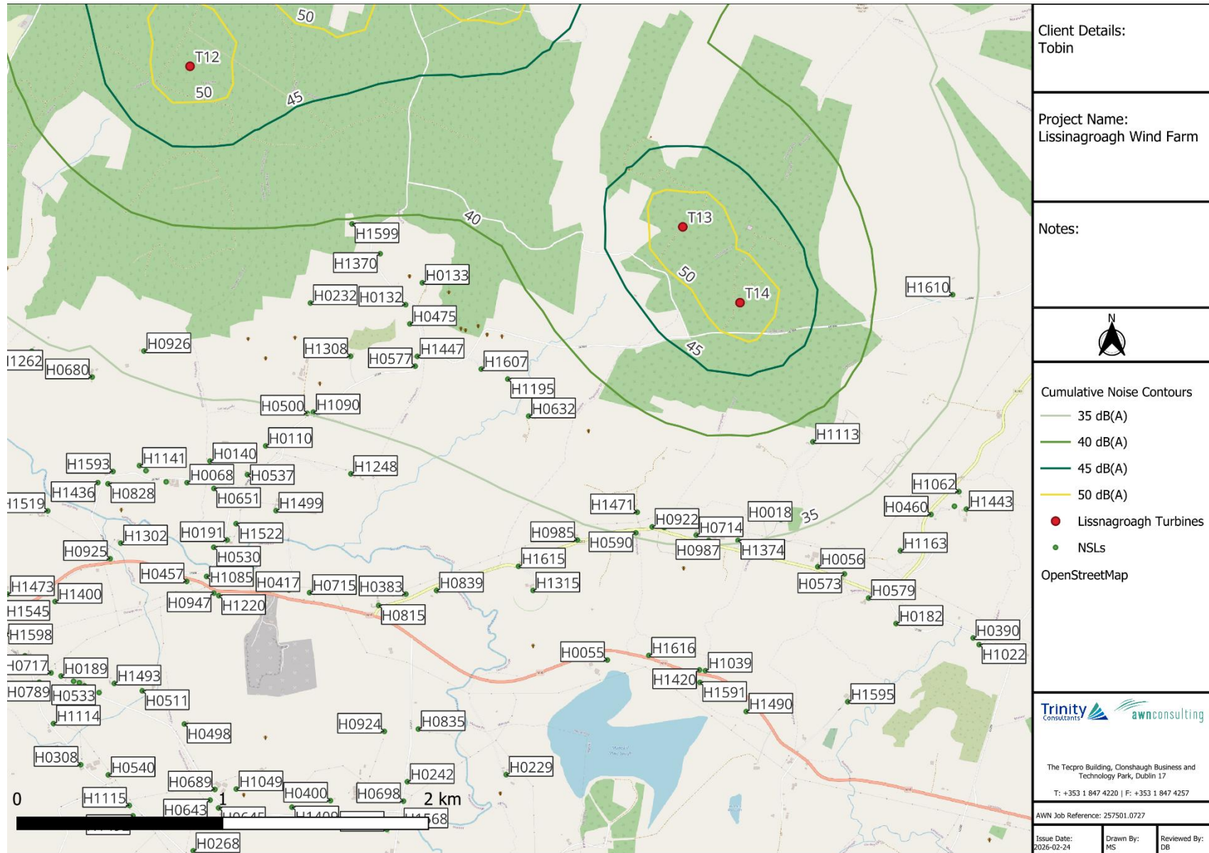
Figure 12-8-5. Predicted Cumulative Noise Contours Detail 4
