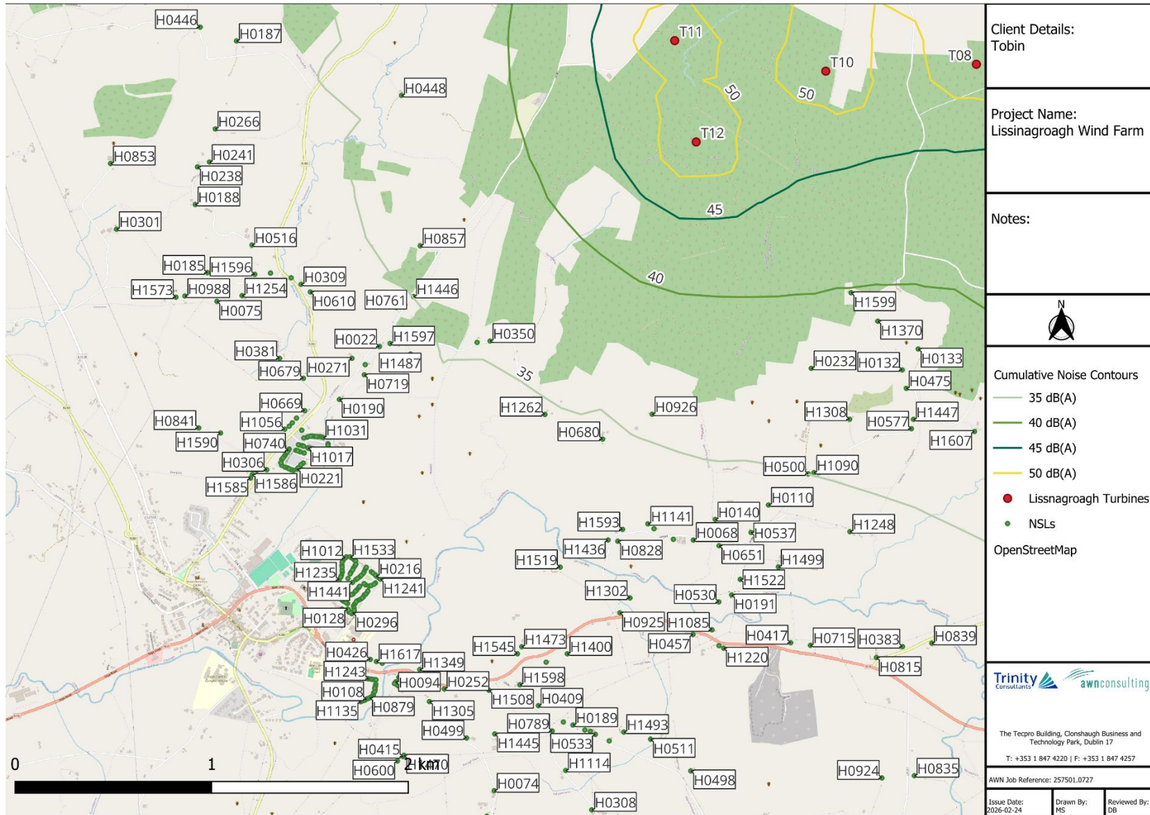
Figure 12-7-4. Predicted Cumulative Noise Contours Detail 3
